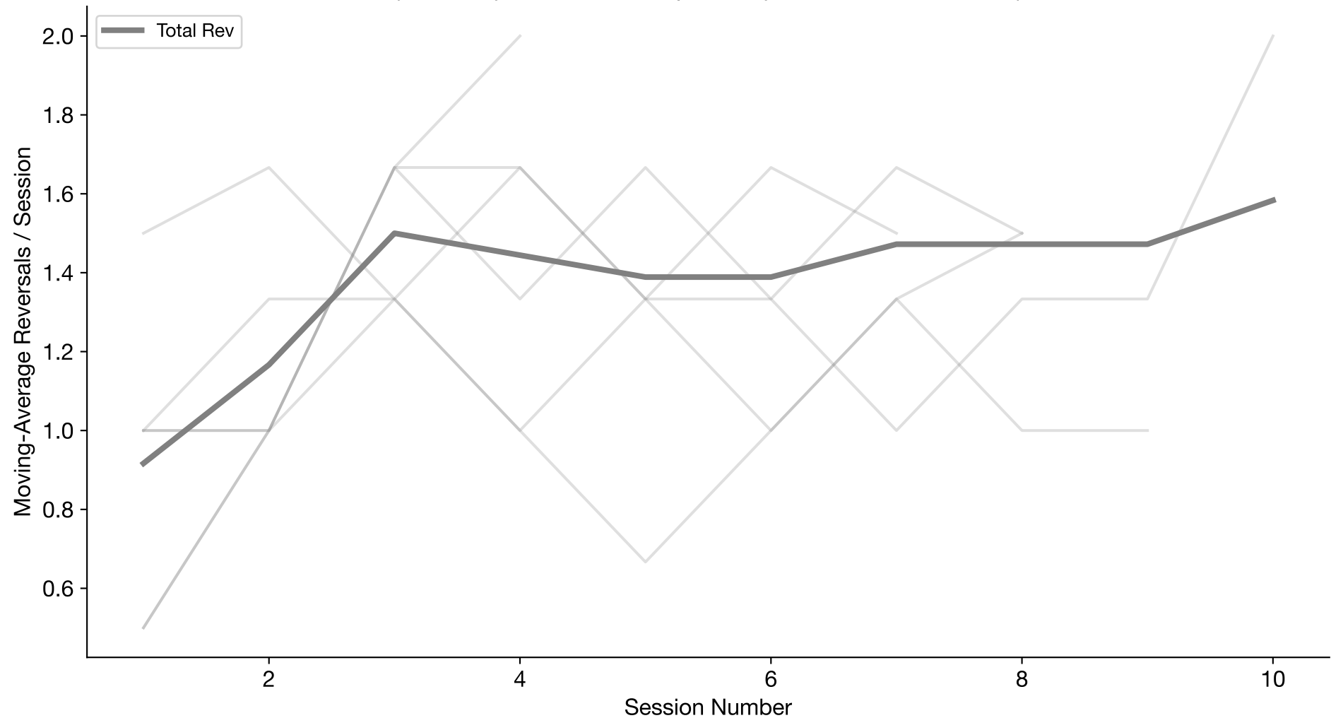
Moving-Average Total Reversals Over Time (n=6 subjects; sessions per subject=4–10; window=3)
